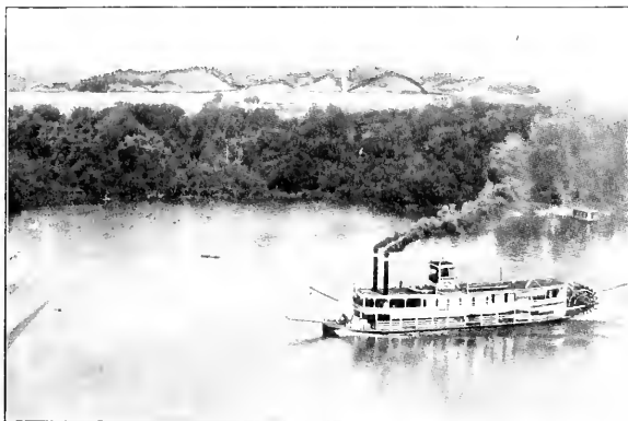
A. View of Illinois Valley north of Peoria, showing terrace and bluffs on east side. (Photo by Dewein.)
